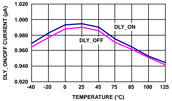
FIGURE 7. DLY CHARGE CURRENT
